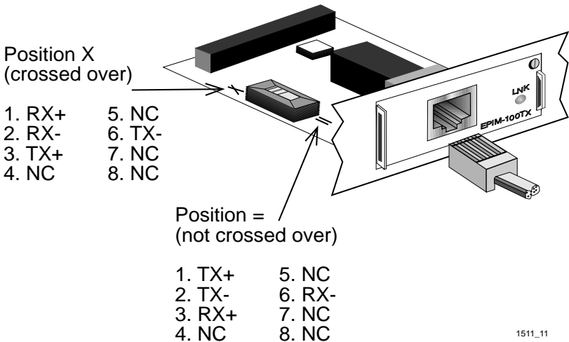
Figure A-1 EPIM-100TX Pinouts
